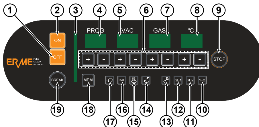
Imm. 5: Centralina CP-E5
