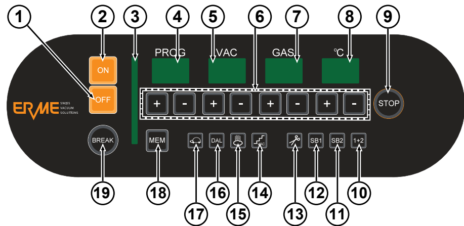
Fig. 14: Controller CP-E5
