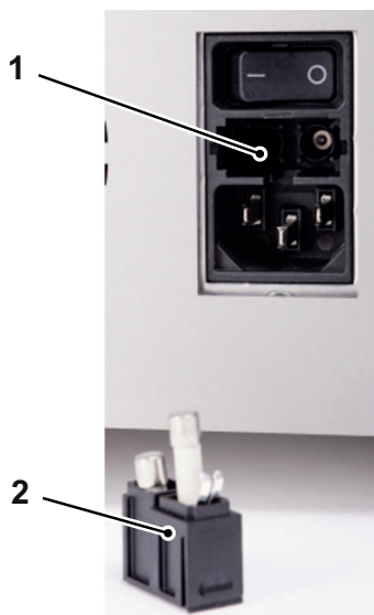
Fig. 18: Fusible
